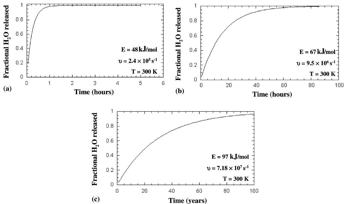
Fig. 7. The simulated release of H 2 O from LiOH · H 2 O structures (a) and (b) and the decomposition of the LiOH structure with E = 97 \text{ kJ/mol} at room temperature (c).
